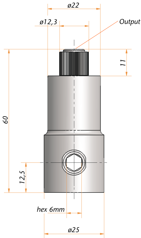
Housing made of zinc diecasting
